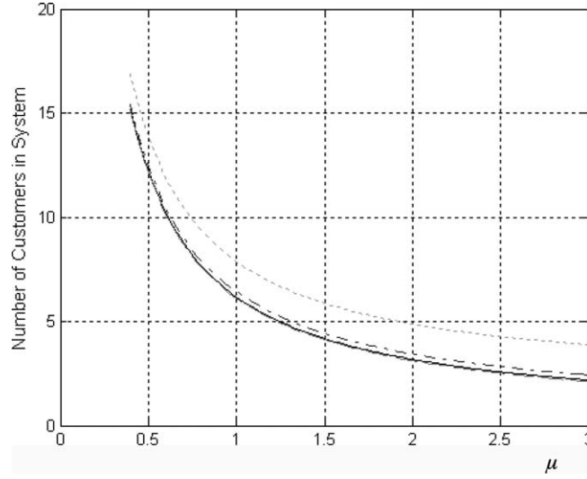
Figure 1. Expected number of customers in the system with \mu = 3\mu' . (--- f = 0.005, r = 0.05 ; — f = 0.002, r = 0.05 ; -- f = 0.002, r = 0.075 ; ... f = 0.05, r = 0.075 ).
