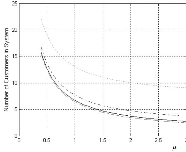
Figure 2. Expected number of customers in the system with \mu = 10\mu' . (--- f = 0.005, r = 0.05 ; — f = 0.002, r = 0.05 ; -- f = 0.002, r = 0.075 ; ... f = 0.05, r = 0.075 ).
